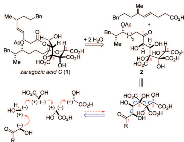
Figure 2. Retrosynthetic analysis.
